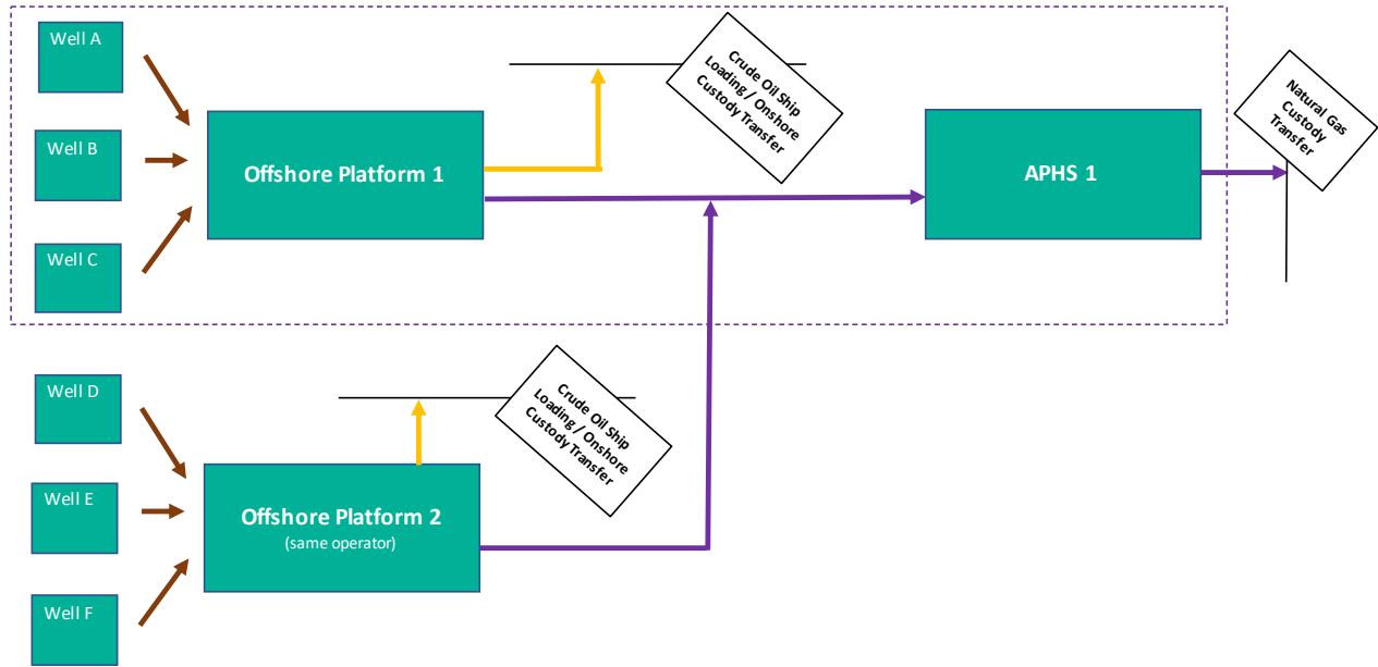
Figure 2: Facility boundary of Offshore Platform 1 ending at the custody transfer metering point downstream of Auxiliary Product Handling Site (APHS) 1, which is owned and operated by the operator of Offshore Platform 1 and does not handle any significant (>50% of Facility Throughput) third-party flows.
